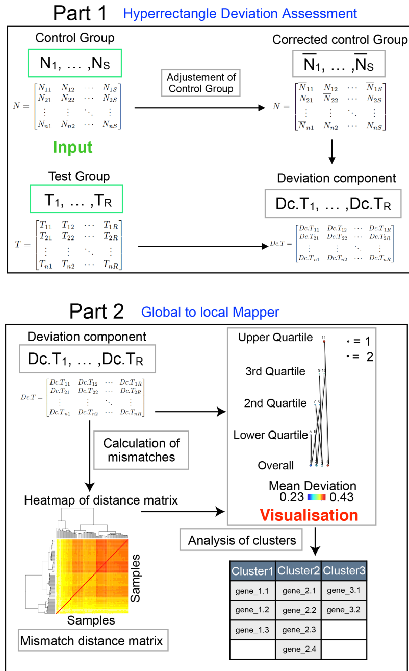
Figure 1: Schematic overview of TMap. The inputs (green) are given by two gene expression matrices, the control (N) and the test group (T), rows represent genes and columns samples. In Part 1, TMap adjusts the control group for outlier values ( \bar{N}_* ), feature by feature. It calculates deviation from this corrected control group for individual samples in the test group ( Dc.T_* ). In Part 2, TMap computes a similarity measure, the mismatch distance (represented as a heatmap) using the deviation components. The Mapper [?] algorithm is used with a two-tier cover to generate a visual representation of the clustering creating a network of global clusters (Overall) and local clusters (1st, 2nd, 3rd, 4th quartile of a filter function). It takes as inputs the mismatch distance and the deviation components.
